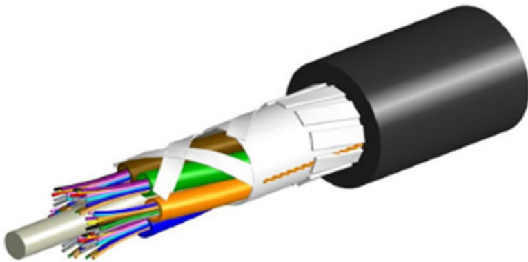
Indoor/Outdoor LSZH Mini Single Jacket Cable for indoor or outdoor use
