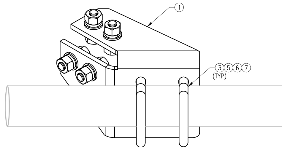
4-SIDED SUPPORT RAIL CORNER BRACKET ISOMETRIC VIEW
