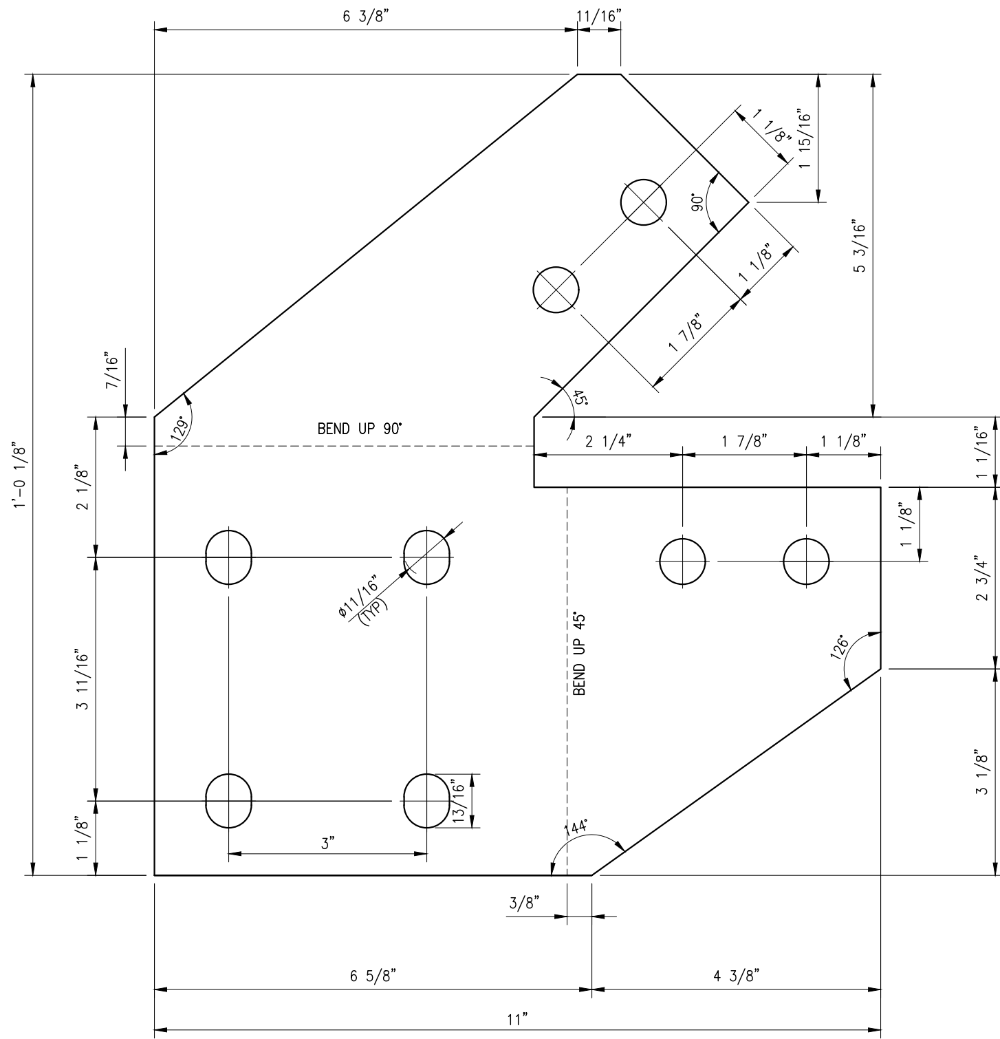
BEFORE BENDING
