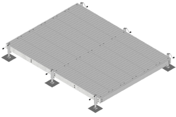
Equipment Platform, 12 ft x 14 ft, base with six adjustable legs
