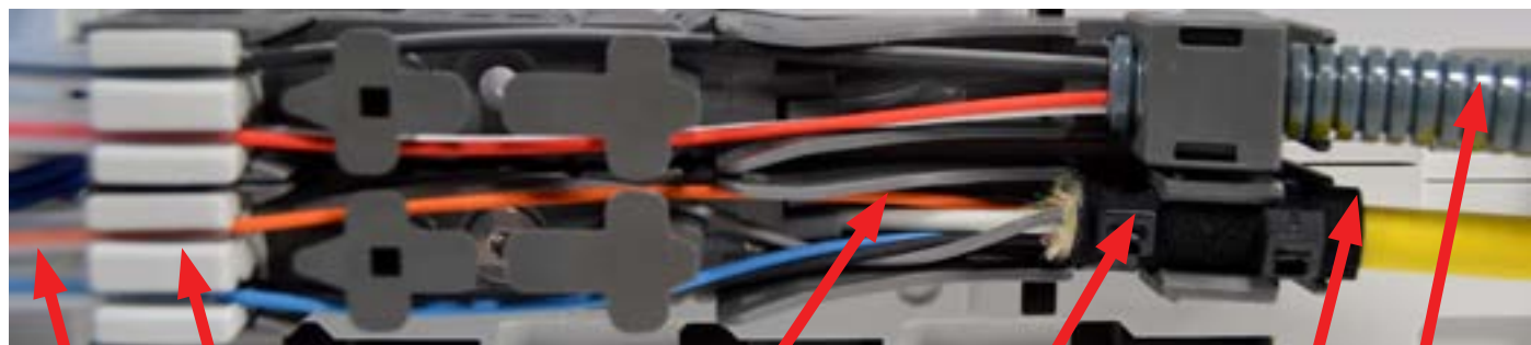
Fopt tube Fopt tube holder Strength member Foam + Tie Wraps Fiber Cable / Flex Tube
