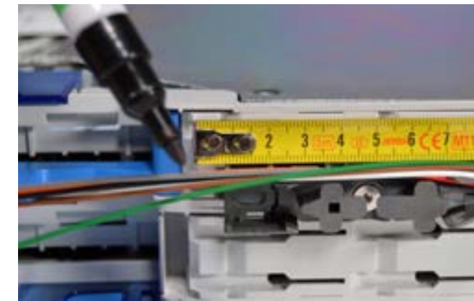
7.1.1. Slide on the CTU bracket. Mark the loose tubes at 1 cm from the CTU bracket.
