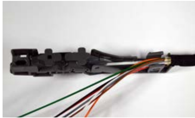
5.3.2. Feed the strength member to the backside.
