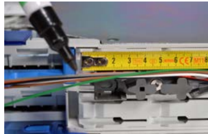
6.1.1. Slide on the CTU bracket. Mark the loose tubes at 1 cm of the tube holder.
