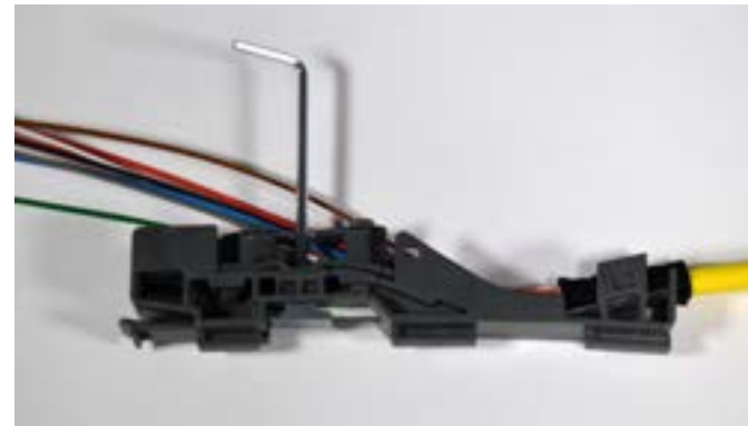
5.3.3. Fix the strength member, using the Allen key.
