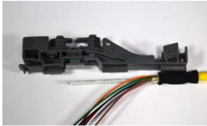
5.3.1. Cut the strength member on length +/- 70 mm.
