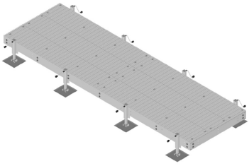
E20® Equipment Platform, 4 ft x 20 ft, base with eight adjustable legs
