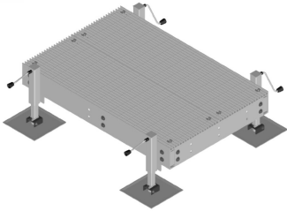
Equipment Platform, 4 ft x 6 ft, base with four adjustable legs
