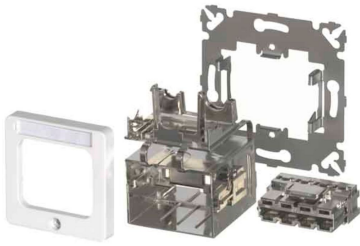
AMP CO Ultra Outlet Installation Kit, shielded, flush mount, DIN 50 x 50, almond
