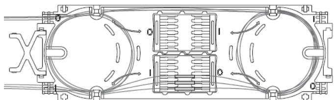
End Storage Routing
