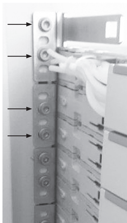
3.1 Final position of the cage nuts for 2 element brackets
