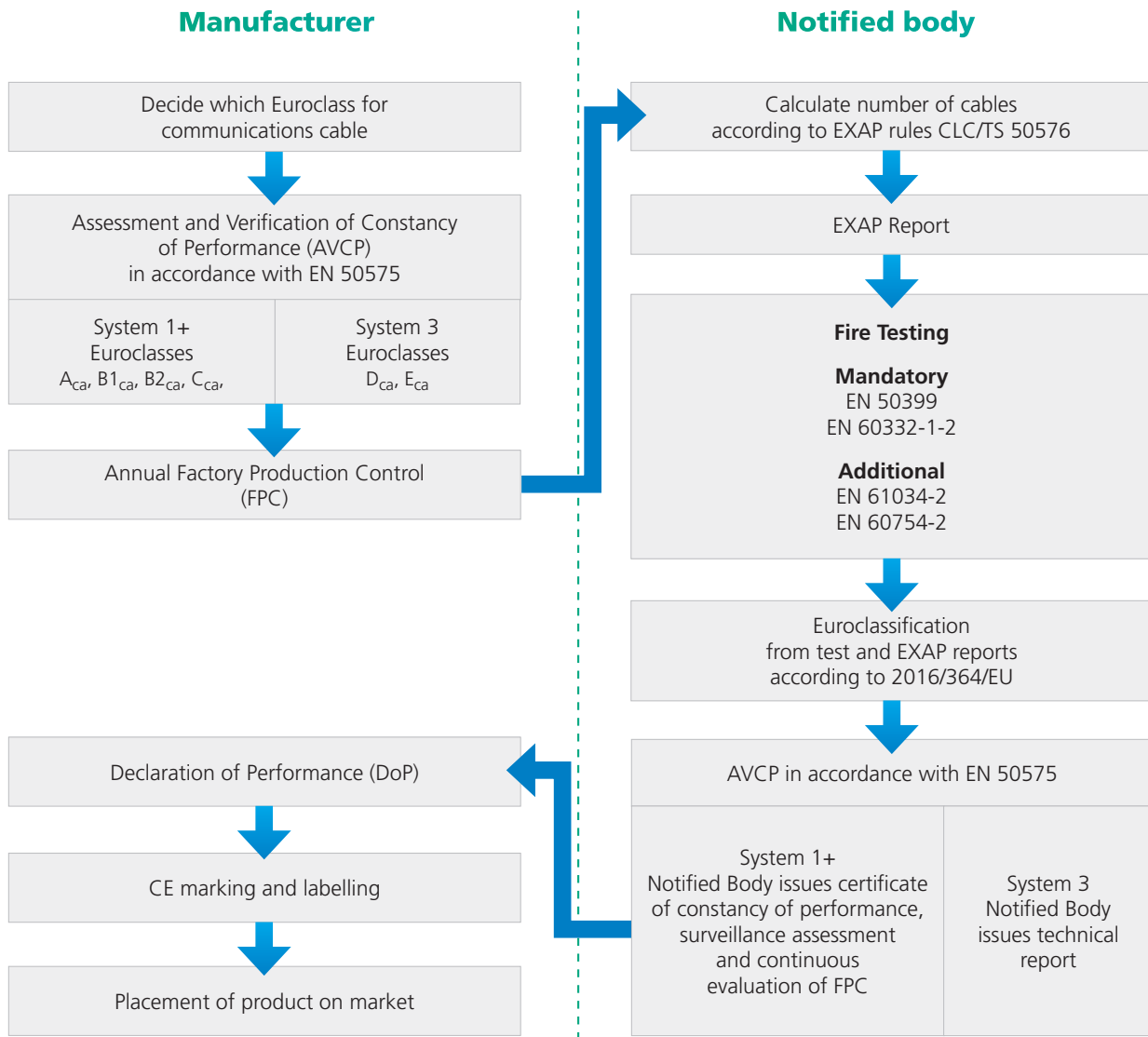
Figure 1: Procedures for CE marking of communications cables
