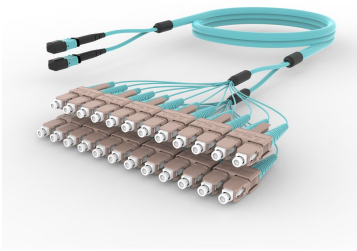
OM3 MPO (Pinned) to SC/UPC, InstaPATCH® 360 Ruggedized Fanout Cable, 24-Fiber, Plenum
