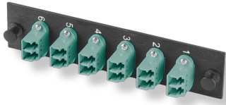
Fiber Optic Adapter Pack, multimode, LC, duplex, 12-port, aqua
