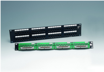
PowerSUM 2500 Category 5 U/UTP Patch Panel, 24 port A wiring
