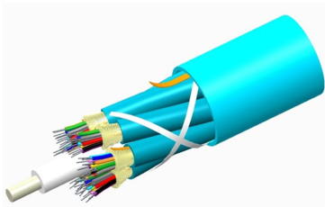
LazrSPEED® Plenum Distribution Cable, 48 fiber multi-unit with 12 fiber subunits
