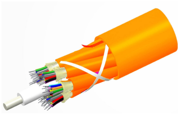
TeraSPEED® Plenum Distribution Cable, 96 fiber multi-unit with 12 fiber subunits
